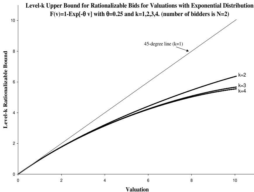
Figure 9: Level-k rationalizable bounds \bar{B}_k(\cdot; \mathcal{N}) for F_0(v) = 1 - e^{-0.25v} , \mathcal{N} = 2 and k = 1, 2, 3, 4 .
