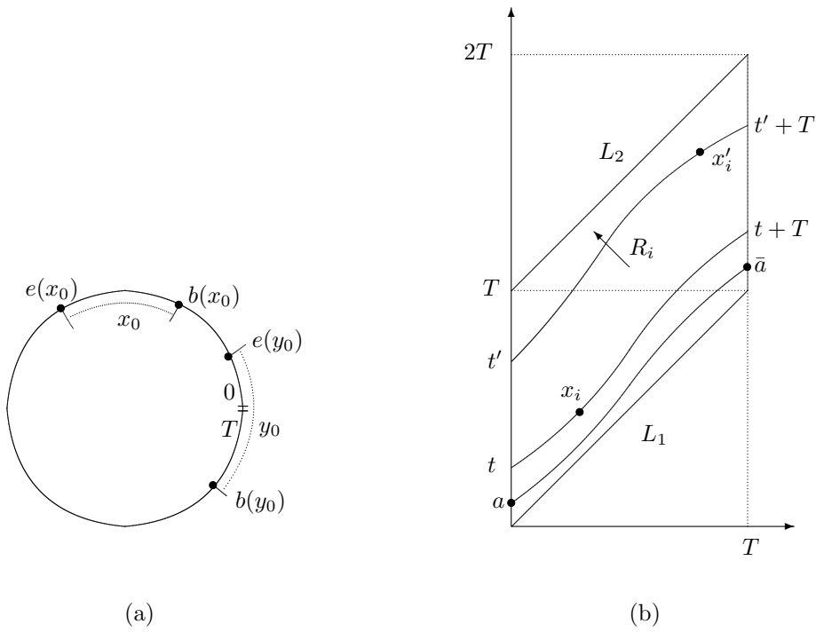
Figure 1: Partitioning a circle into arcs. (a) Arcs are measured counterclockwise from the origin marked 0. (b) Representation in \mathbb{R}_+^2 of a preference relation over arcs.
