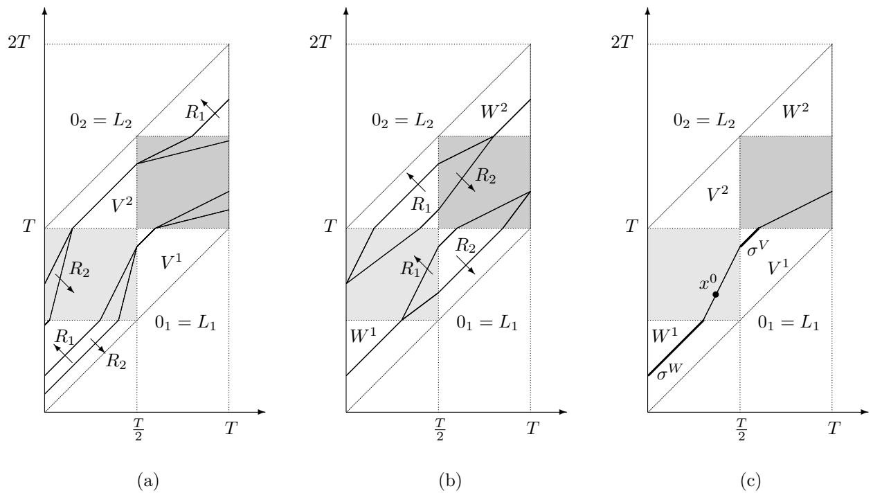
Figure 9: Strategy-proofness for additive preferences. Step 1 of Theorem 7. There are three possible shapes for the Pareto set.
