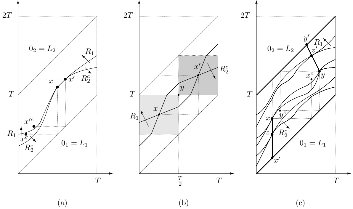
Figure 7: Relating no-envy and efficiency (Theorem 2). Panels (a), (b), (c) illustrate parts (a), (b), and (c) of the theorem.
