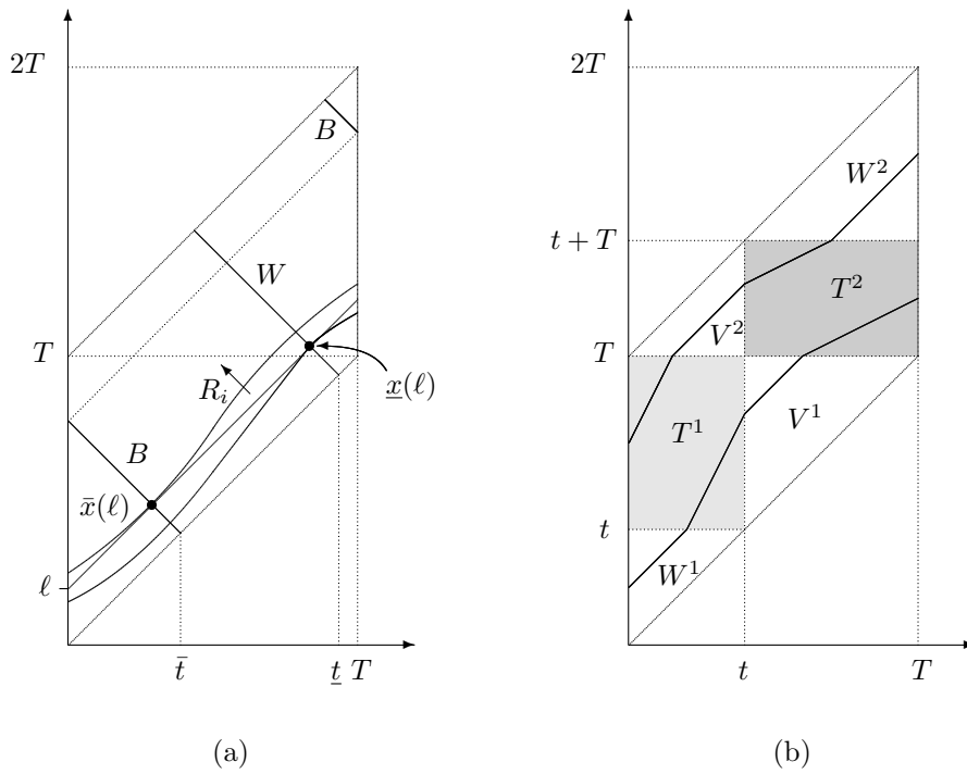
Figure 2: Special maps. (a) A notion of single-peaked preferences. (b) Additive preferences relative to a two-component partition of the circle.
