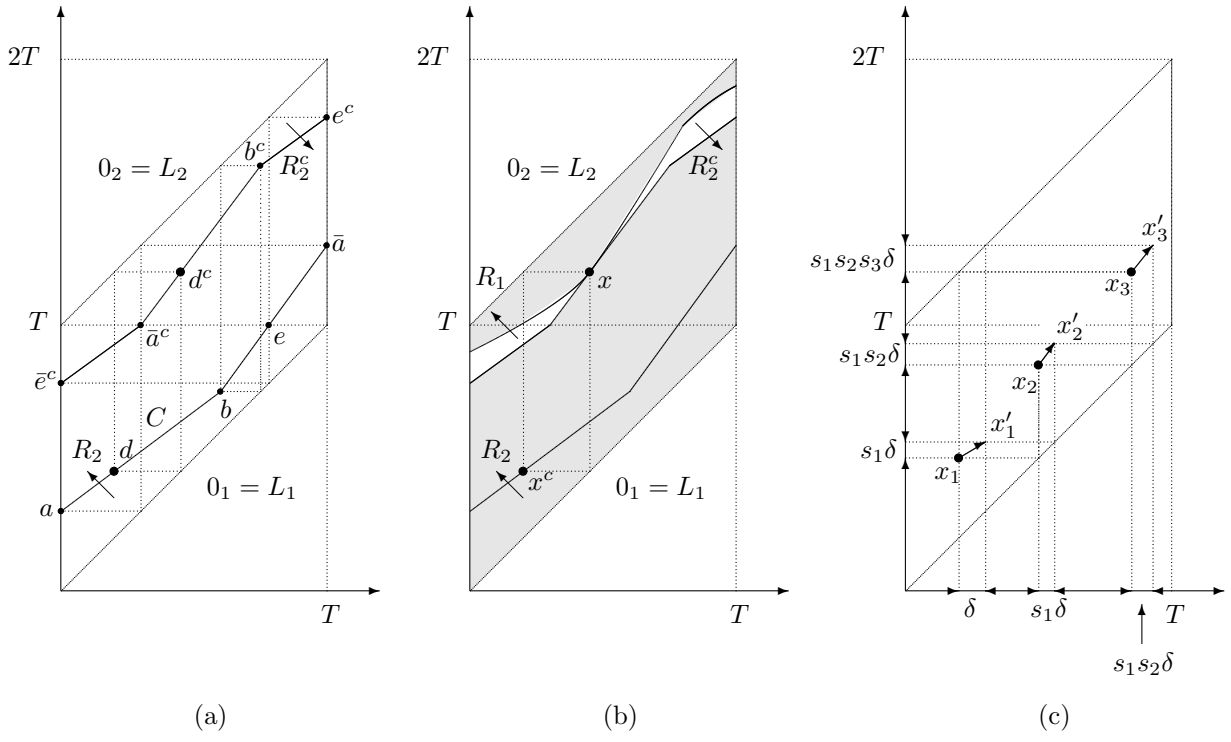
Figure 4: Pareto efficient partitions. (a) Calculating the “complement” of a typical indifference curve of agent 2. (b) Efficiency for |N| = 2 . By maximizing agent 1’s preferences over the complement of a typical indifference curve of agent 2’s, we obtain an efficient partition. (c) Efficiency for general |N| .
