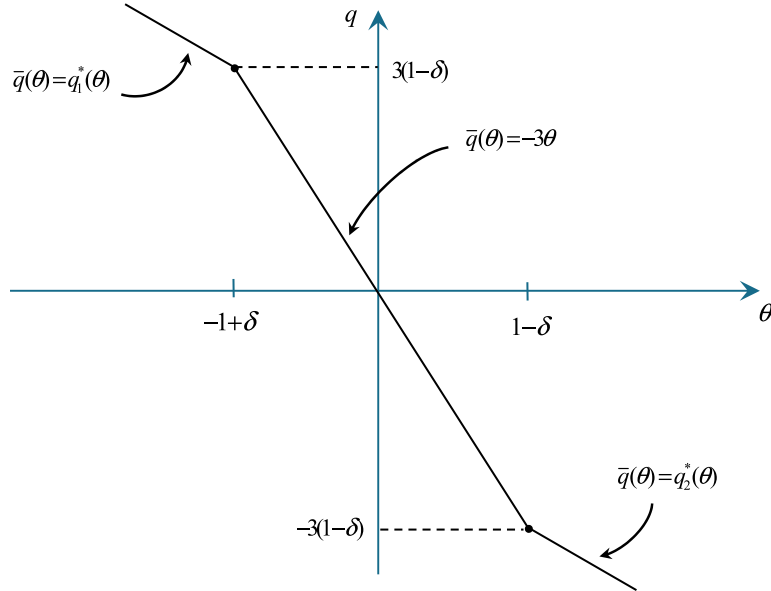
Figure 2: Virtually-truthful equilibrium allocation in a symmetric lobbying game, s_1 = -s_2 = 1 , with \delta \in (\frac{1}{2}, 1) . Common influence arises for types \theta \in (\delta - 1, 1 - \delta) .
